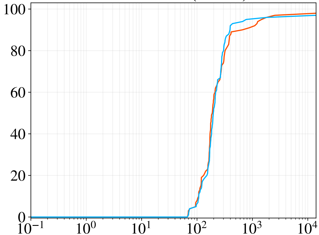
Time (seconds)
