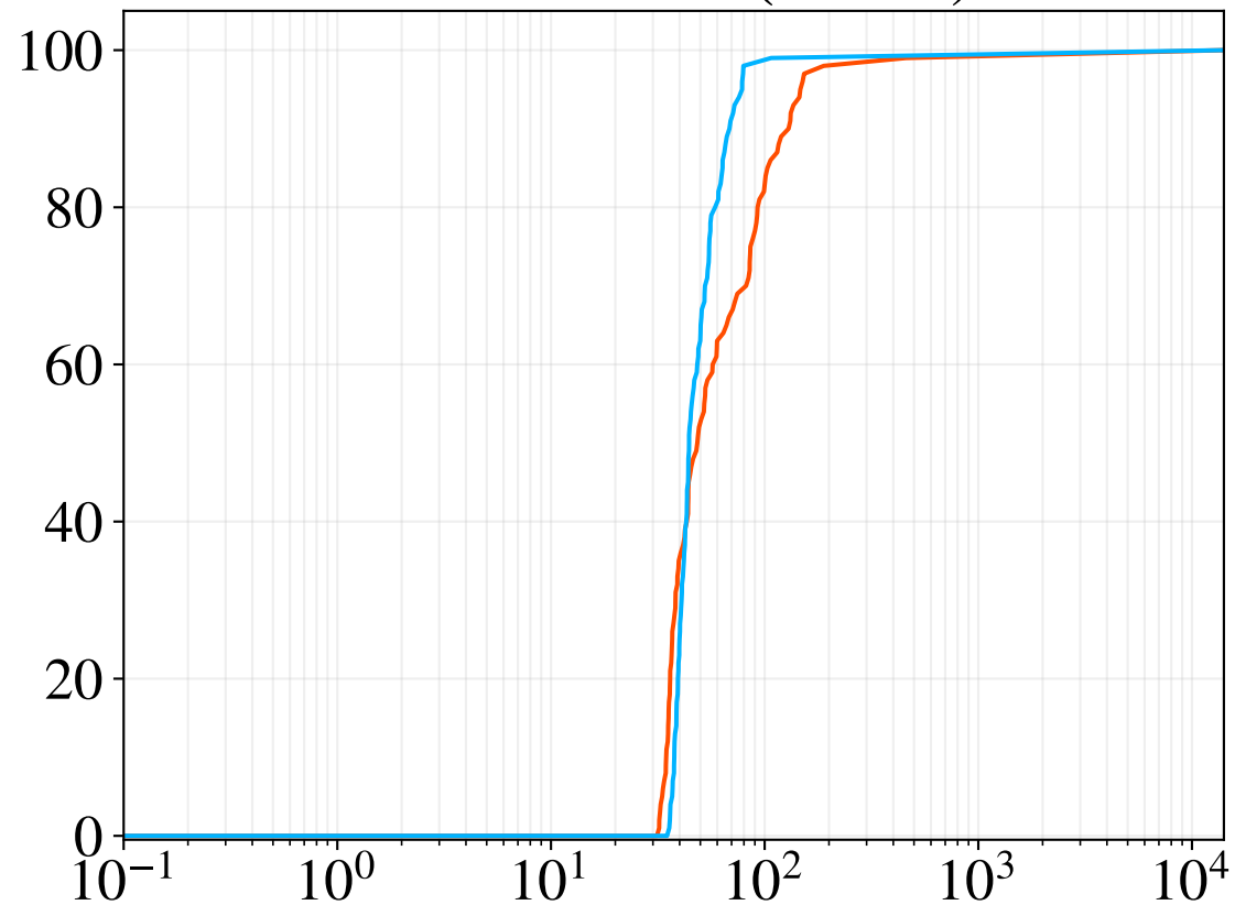
Performance (5x100)
