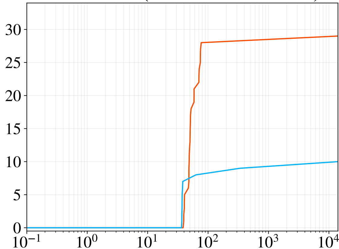
Peformance (ReluBilinearSoftmax)
