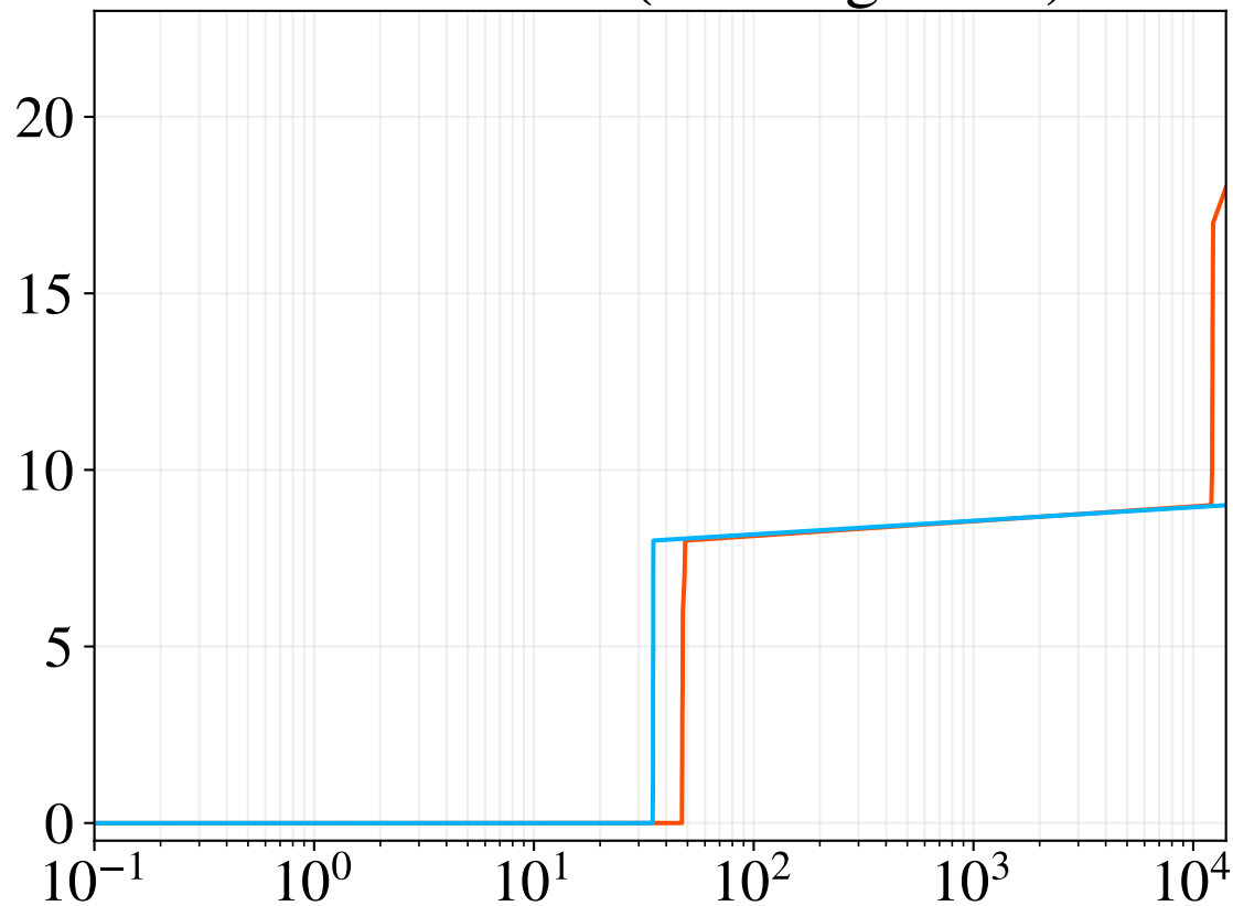
Performance (ReluSignMax)
