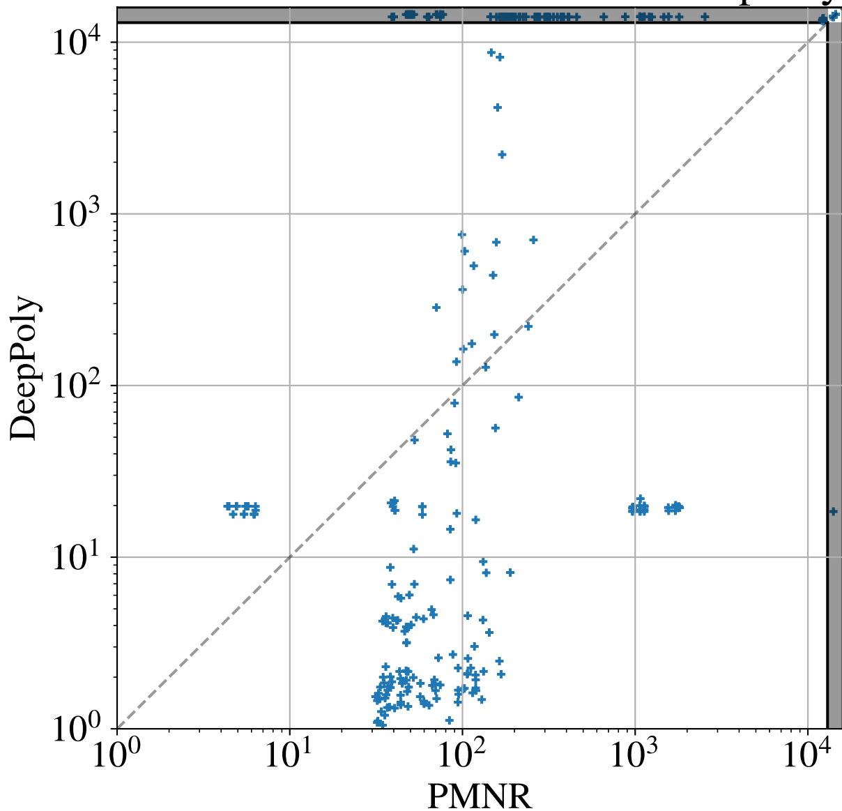
Performance of PMNR versus DeepPoly
