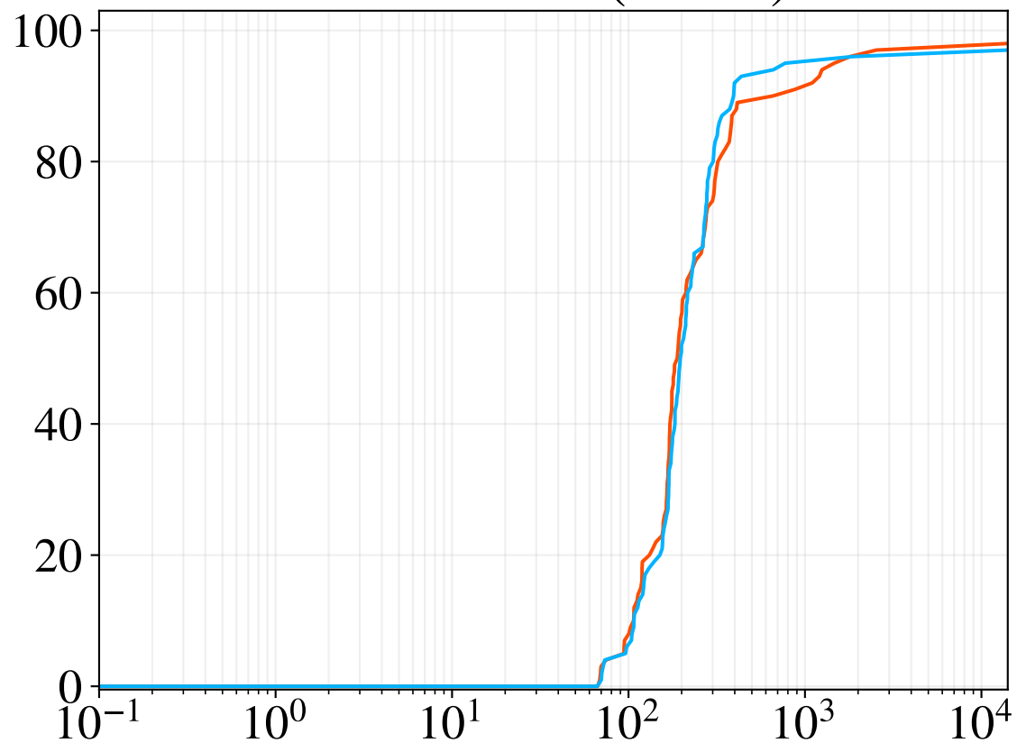
Peformance (8x100)
