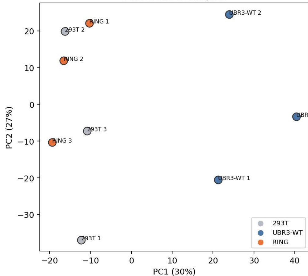
PCA of the 9 samples
