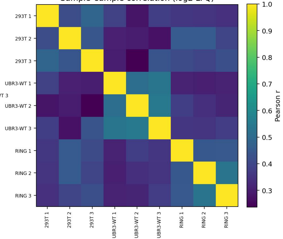
Sample-sample correlation (log2 LFQ)
