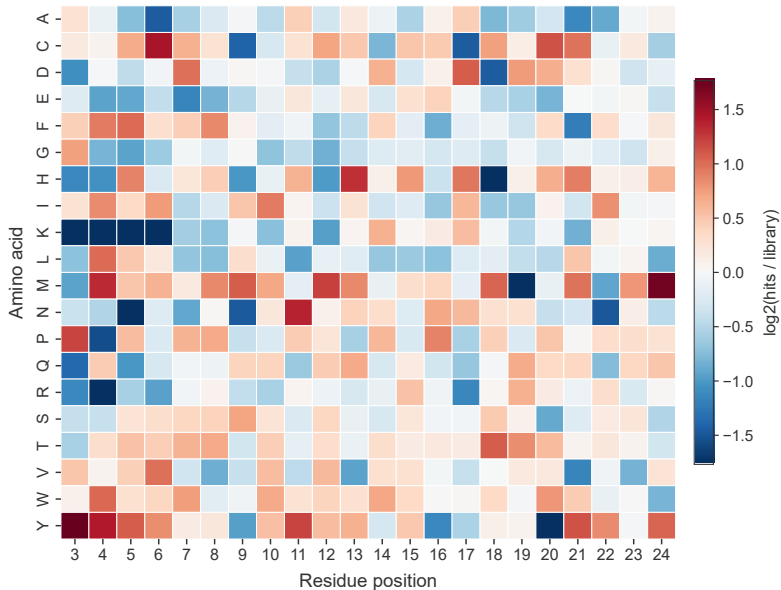
Enrichment heatmap (hits / full library)
