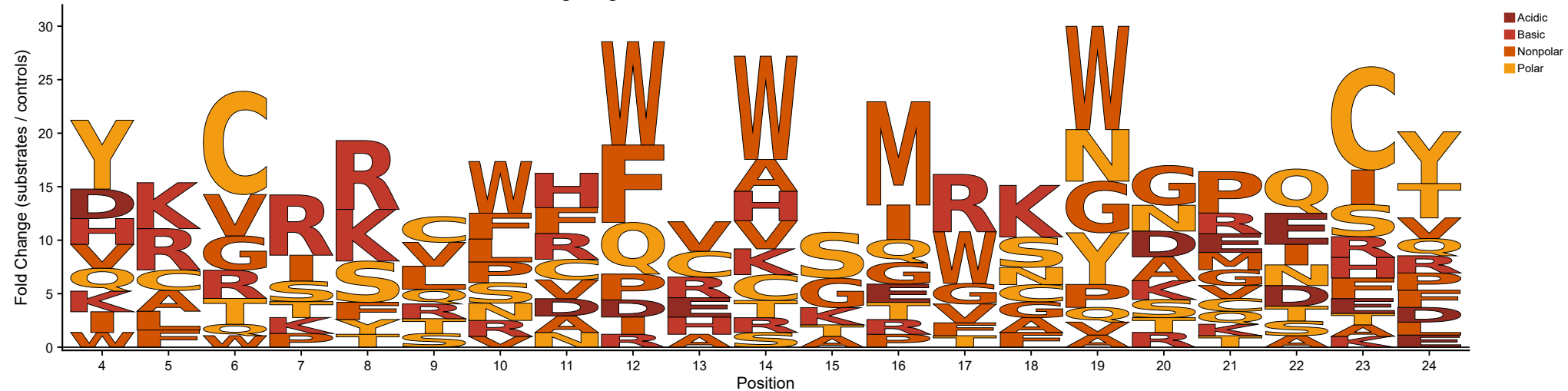
Fold-Change Logo — P/G-D/E/T Substrates vs Non-Substrate Controls
