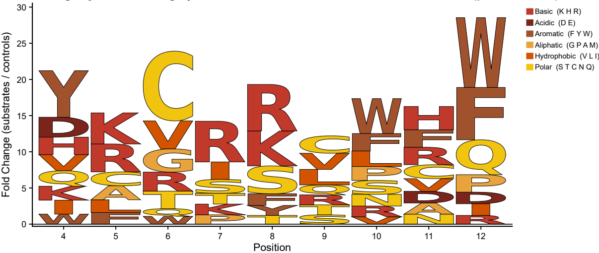
Enrichment Logo by Residue Category — P/G-D/E/T Substrates vs Non-Substrate Controls (positions 4–12)
