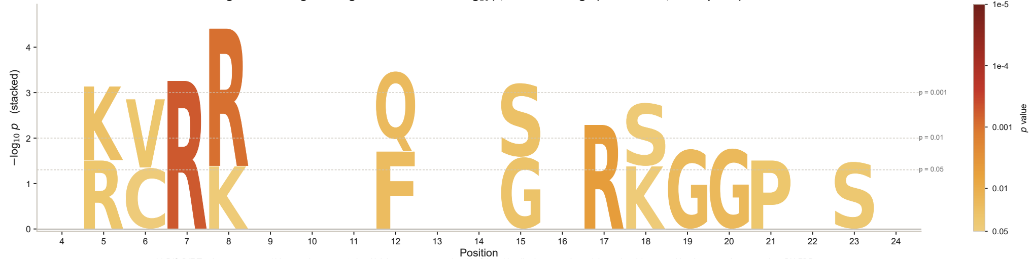
Significance Logo — height and colour are -\log_{10} p , not fold change (Fisher exact, recomputed)
