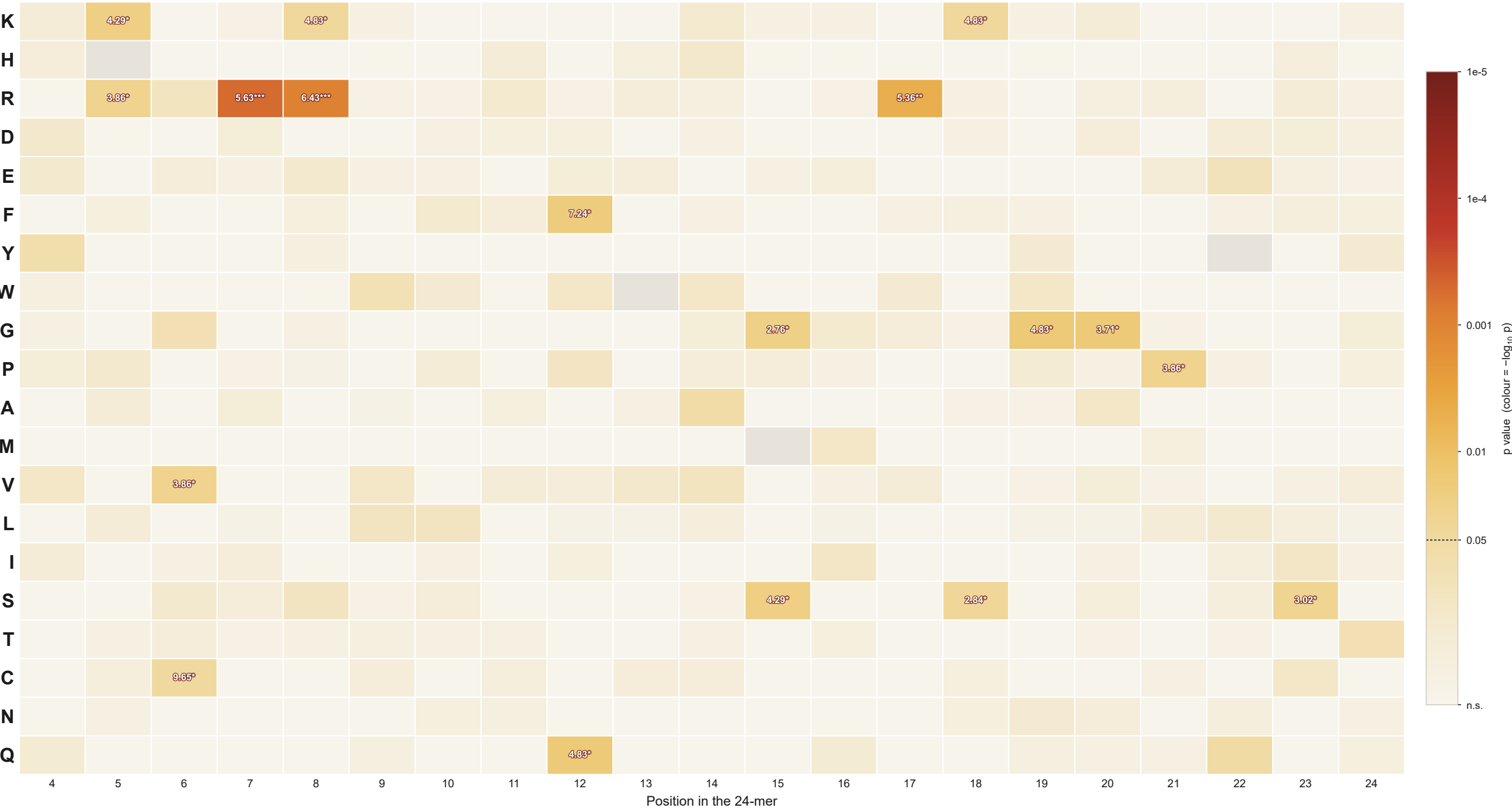
Position × residue enrichment, coloured by significance (Fisher exact) colour = -\log_{10} p , Fisher exact recomputed from the same 2×2 tables — valid at the low cell counts here
