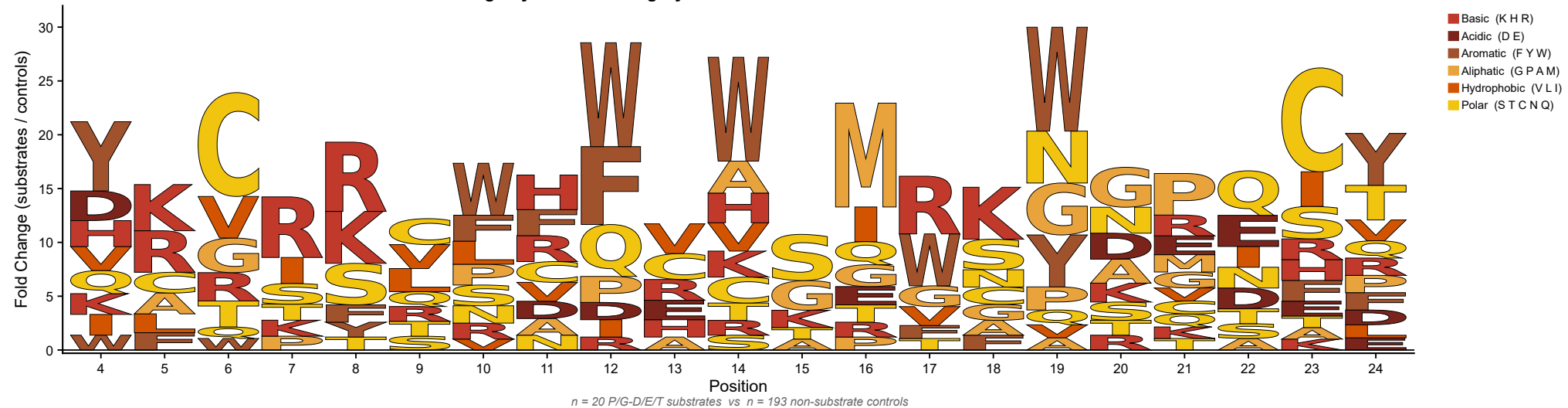
Enrichment Logo by Residue Category — P/G-D/E/T Substrates vs Non-Substrate Controls
