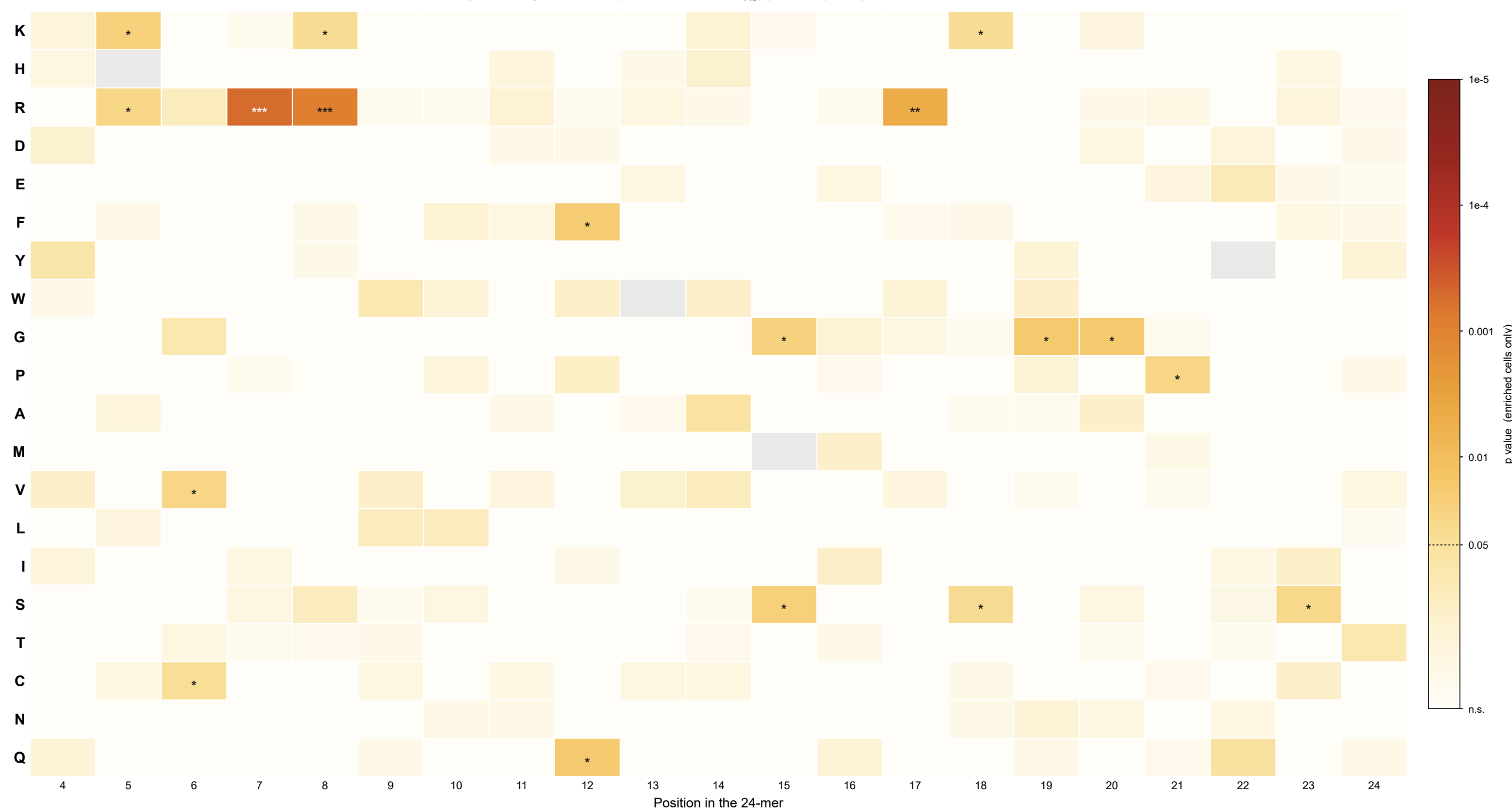
Position × residue enrichment, coloured by significance (enriched cells only) same layout as the original Colab heatmap, but the colour scale is -\log_{10} p (Fisher exact) and depleted cells are held at the floor
