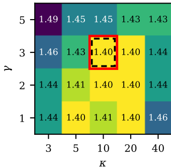
CIFAR-100
