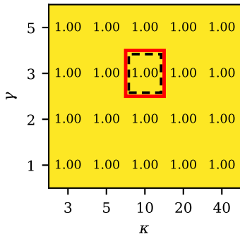
CIFAR-10
