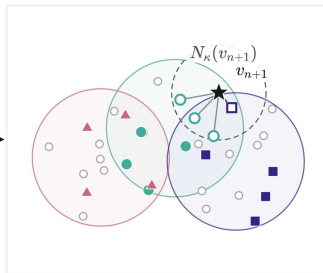
(b) whitened v = \tilde{\Sigma}^{-1/2} V^{\top} (x - \mu_{\mathcal{U}})
