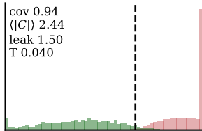
CIFAR-100
