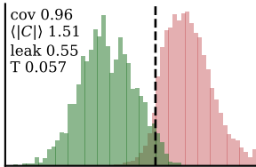
CIFAR-10
