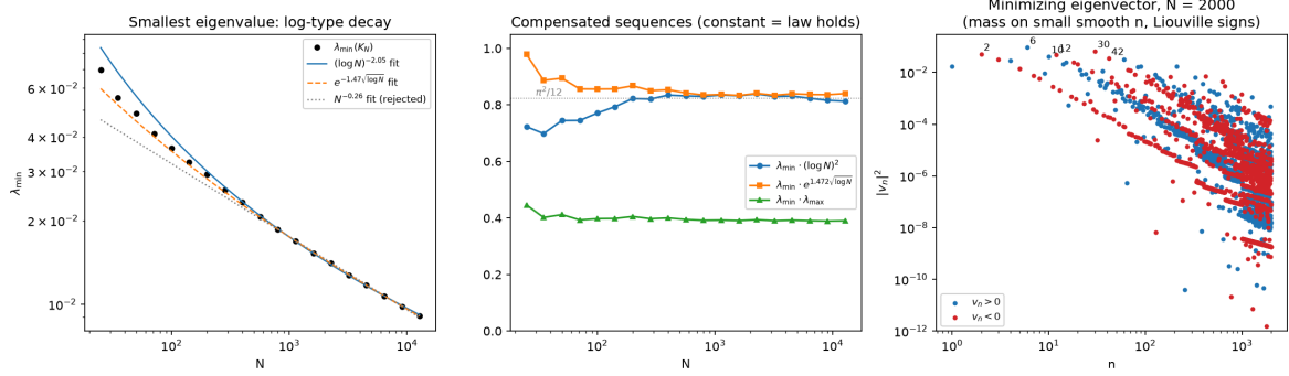
Figure 1: The dense-spectrum window N \leq 25\,600 . Left: \lambda_{\min}(N) with fitted laws; the fixed power of N is rejected. Middle: compensated sequences for the two surviving two-parameter laws. Right: the minimizing eigenvector at N = 2000 , with mass on small smooth n and signs following the Liouville function.
