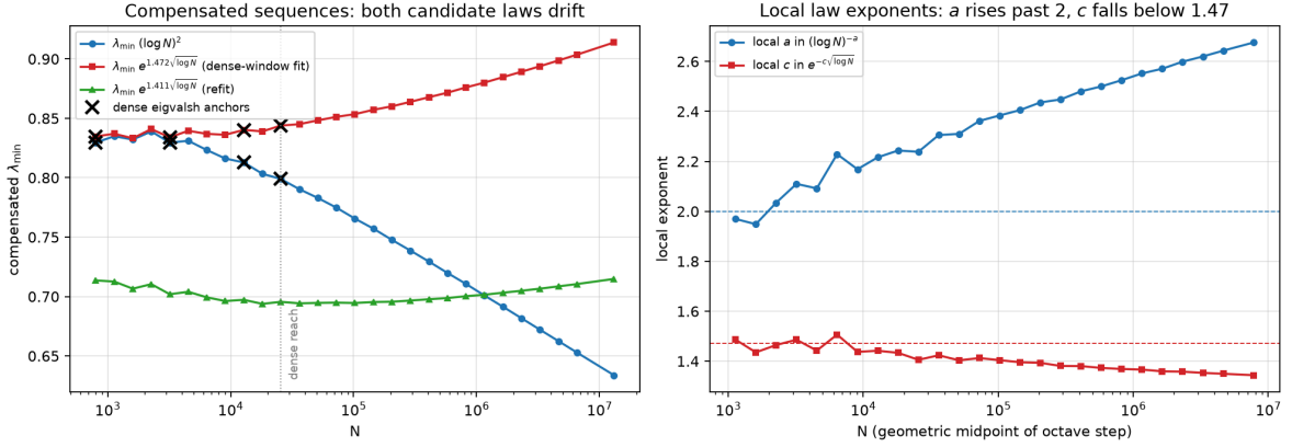
Figure 2: The Lanczos extension, 800 \leq N \leq 1.3 \times 10^7 , via the exact Möbius-sparse inverse. Left: both two-parameter candidate laws drift; \lambda_{\min}(\log N)^2 falls with no flattening while the dense-window-calibrated exponential compensation rises slowly. Crosses mark dense eigvalsh anchors. Right: the local log-power exponent rises past 2 as the exponential law forces, while the local exponential rate drifts slowly below 1.47.
