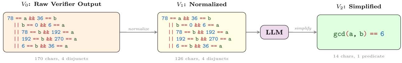
Figure 1: WONDA pipeline on 187_1.c. The raw verifier output ( V_0 ) is normalized ( V_1 ); the LLM then unifies enumerated Euclid states into one constant GCD constraint (function-call form) ( V_2 ): gcd(a, b) == 6 , a 12× character reduction with 35.5× verification speedup.
