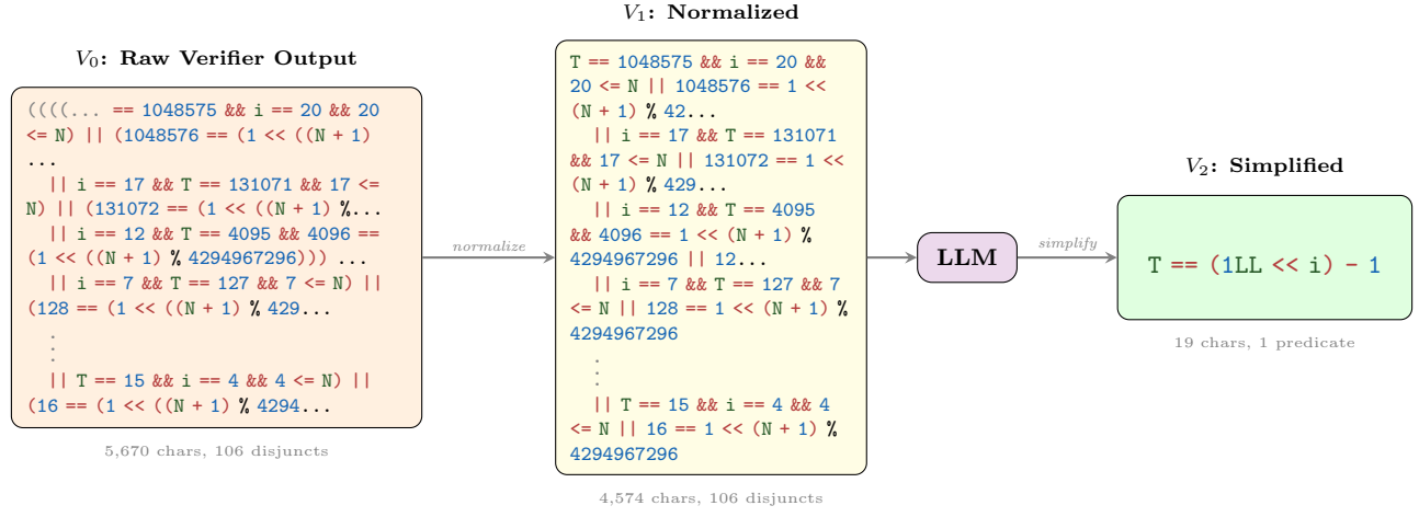
Figure 1: WONDA pipeline on 2148_1.c. The raw verifier output ( V_0 ) is normalized ( V_1 ); the LLM then states the bitwise-accumulation closed form and drops redundant modulo constraints ( V_2 ): T == (1LL \ll i) - 1 , a 298× character reduction with 1.5× verification speedup.
