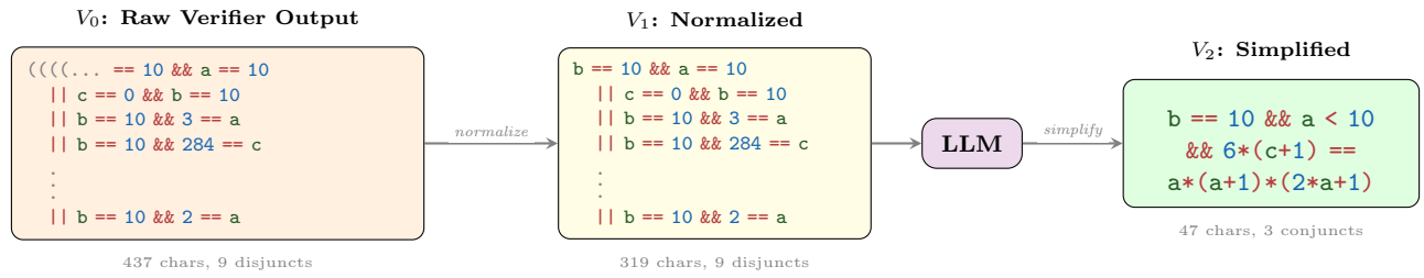
Figure 1: WONDA pipeline on 2686_1.c. The raw verifier output ( V_0 ) is normalized ( V_1 ); the LLM then replaces per-value case enumeration with a sum-of-squares closed form ( V_2 ): b == 10 && a < 10 && 6*(c+1) == a*(a+1)*(2*a+1) , a 9\times character reduction with verified correct & sufficient.
