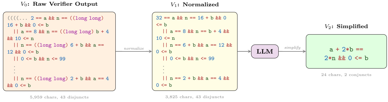
Figure 1: WONDA pipeline on 274_1.c. The raw verifier output ( V_0 ) is normalized ( V_1 ); the LLM then captures the loop’s fixed linear update law and a needed non-negativity bound ( V_2 ): a + 2*b == 2*n \ \&\& \ 0 \leq b , a 248× character reduction with 12.5 × verification speedup.
