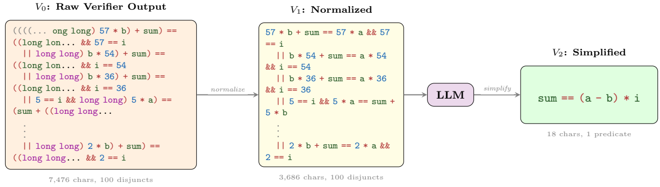
Figure 1: WONDA pipeline on 2953.2.c. The raw verifier output ( V_0 ) is normalized ( V_1 ); the LLM then generalizes enumerated accumulation steps to a single linear counter law ( V_2 ): \text{sum} == (a - b) * i , a 415 \times character reduction with 7.2 \times verification speedup.
