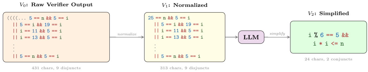
Figure 1: WONDA pipeline on 3197_2.c. The raw verifier output ( V_0 ) is normalized ( V_1 ); the LLM then discards contradictory disjuncts and captures the loop’s stride structure ( V_2 ): i \% 6 == 5 \ \&\& \ i * i \leq n , a 18× character reduction with verified correct & sufficient.
