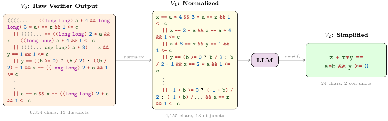
Figure 1: WONDA pipeline on 3917_3.c. The raw verifier output ( V_0 ) is normalized ( V_1 ); the LLM then compresses Russian-peasant-multiplication cases into one preserved product identity ( V_2 ): z + x*y == a*b \ \&\& \ y \geq 0 , a 265× character reduction with 2.8 × verification speedup.
