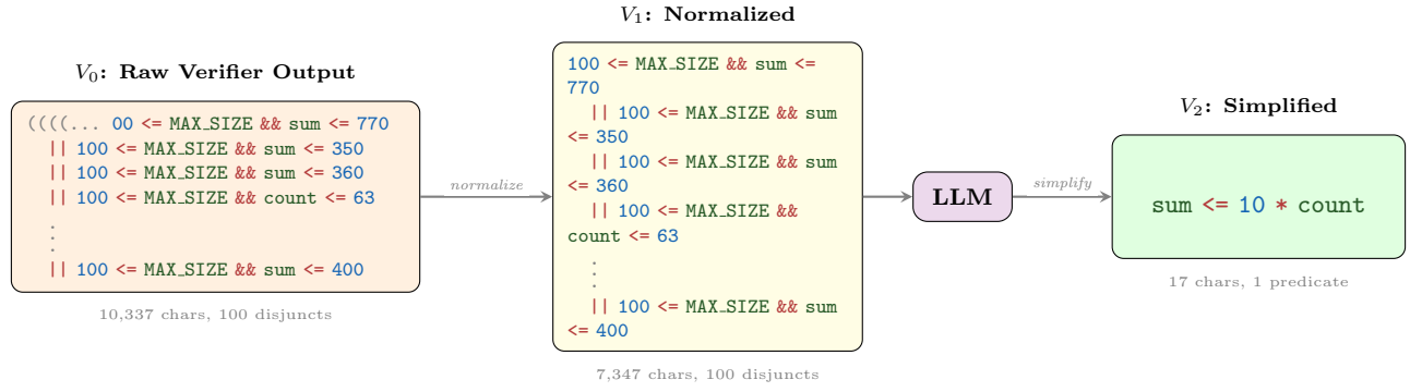
Figure 1: WONDA pipeline on 4820_1.c. The raw verifier output ( V_0 ) is normalized ( V_1 ); the LLM then tightens case-wise sum bounds to the linear inequality implied by each iteration ( V_2 ): sum <= 10 * count , a 608× character reduction with 28.8 × verification speedup.
