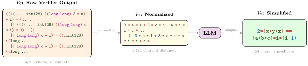
Figure 1: WONDA pipeline on 4828_1.c . The raw verifier output ( V_0 ) is normalized ( V_1 ); the LLM then removes inert conditional branches and states the combined accumulation in linear form ( V_2 ): 2*(x+y+z) == (a+b+c)*i*(i-1) , a 132\times character reduction with 35.9\times verification speedup.
