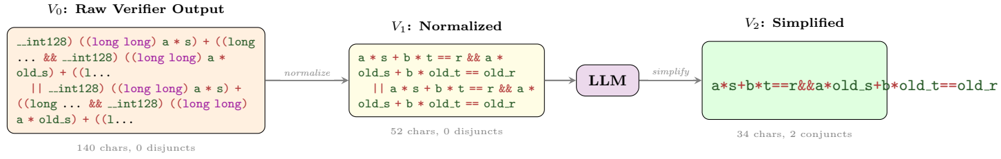
Figure 1: WONDA pipeline on 4992_5.c. The raw verifier output ( V_0 ) is normalized ( V_1 ); the LLM then keeps the essential Bézout linear combinations with minor syntactic compaction ( V_2 ): a*s+b*t==r\&\&a*old\_s+b*old\_t==old\_r , a 4× character reduction with verified correct & sufficient.
