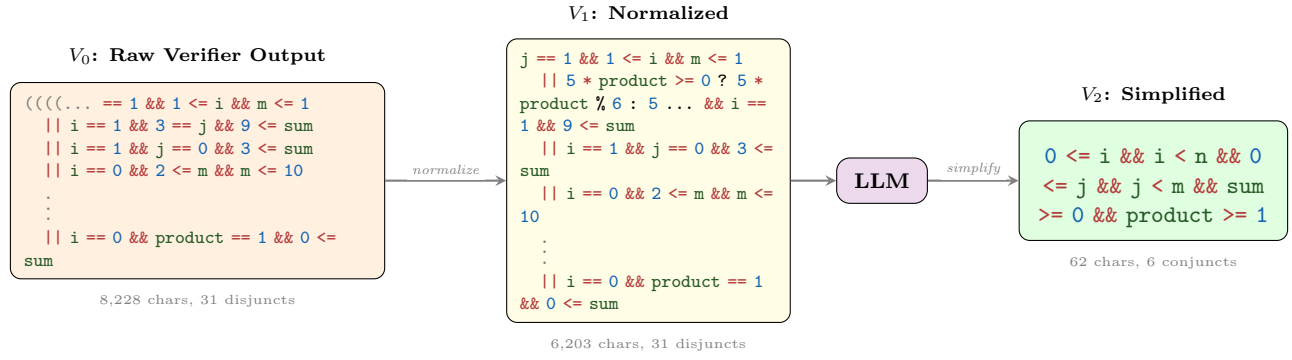
Figure 1: WONDA pipeline on 5066_1.c. The raw verifier output ( V_0 ) is normalized ( V_1 ); the LLM then drops overfitted case constraints and keeps core loop-bound and sign facts ( V_2 ): 0 \leq i \ \&\& \ i < n \ \&\& \ 0 \leq j \ \&\& \ j < m \ \&\& \ sum \geq 0 \ \&\& \ product \geq 1 , a 133\times character reduction with 2.6\times verification speedup.
