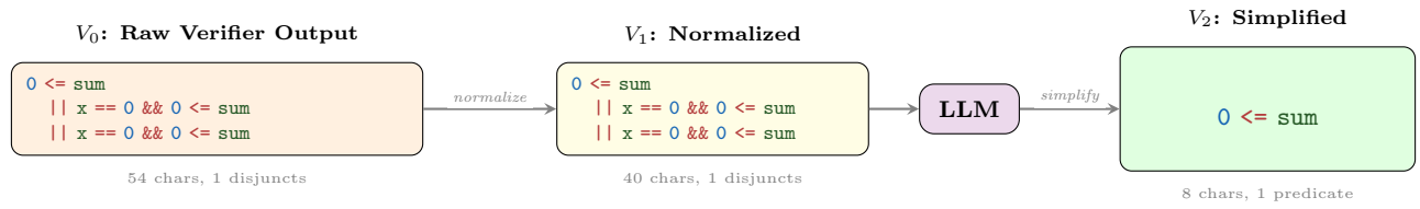
Figure 1: WONDA pipeline on 5582_1.c. The raw verifier output ( V_0 ) is normalized ( V_1 ); the LLM then removes redundant constraints on the loop counter and keeps non-negativity of the sum ( V_2 ): 0 <= sum , a 7\times character reduction with 41.4\times verification speedup.
