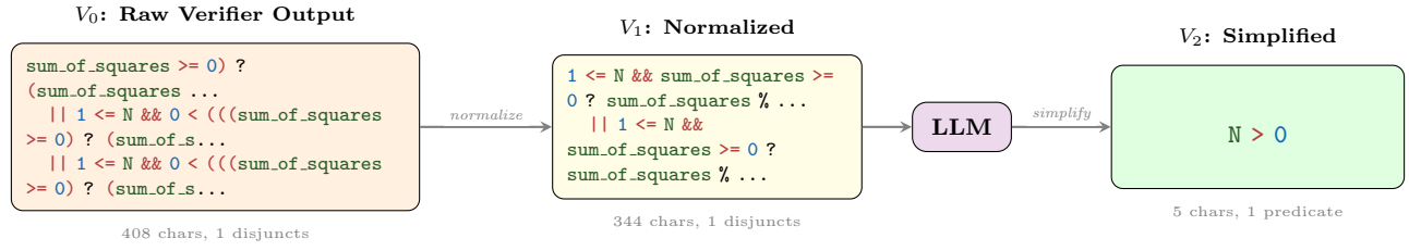
Figure 1: WONDA pipeline on 6098_1.c. The raw verifier output ( V_0 ) is normalized ( V_1 ); the LLM then collapses tautological nested conditionals to the one fact needed for the assertion ( V_2 ): N > 0 , a 82\times character reduction with 1.2\times verification speedup.
