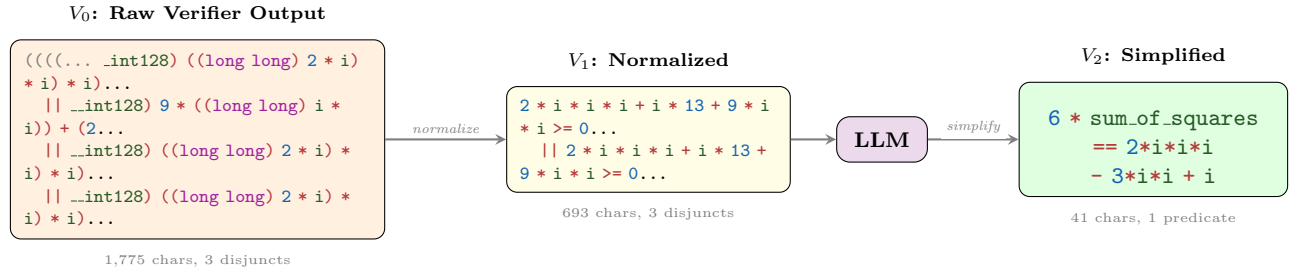
Figure 1: WONDA pipeline on 6732.1.c. The raw verifier output ( V_0 ) is normalized ( V_1 ); the LLM then eliminates floor-division artifacts in favor of an exact polynomial sum-of-squares identity ( V_2 ): 6 * \text{sum\_of\_squares} == 2*i*i*i - 3*i*i + i , a 43\times character reduction with 20.4\times verification speedup.
