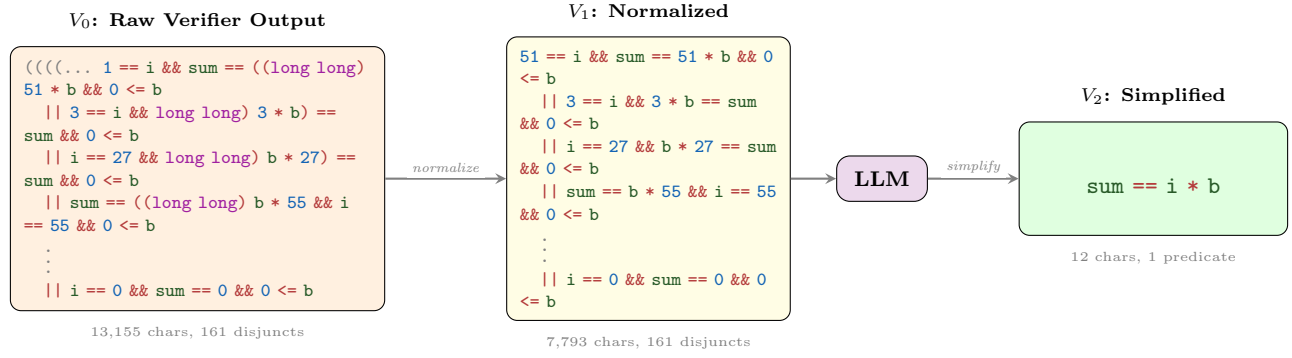
Figure 1: WONDA pipeline on 6858_1.c. The raw verifier output ( V_0 ) is normalized ( V_1 ); the LLM then replaces 161 case-specific disjuncts with the linear accumulation law ( V_2 ): sum == i * b , a 1096× character reduction with 30.2 × verification speedup.
