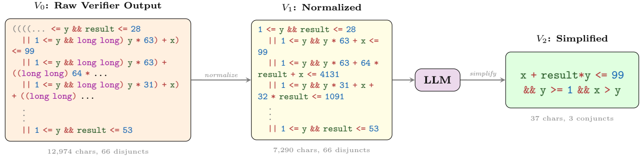
Figure 1: WONDA pipeline on 7158_1.c. The raw verifier output ( V_0 ) is normalized ( V_1 ); the LLM then unifies case-specific bounds into one preserved linear combination ( V_2 ): x + \text{result} \cdot y \leq 99 \ \&\& \ y \geq 1 \ \&\& \ x > y , a 351× character reduction with 21.8 × verification speedup.
