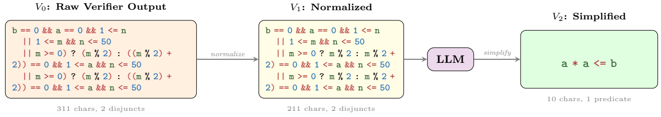
Figure 1: WONDA pipeline on 7241_1.c. The raw verifier output ( V_0 ) is normalized ( V_1 ); the LLM then removes constant and parity constraints that are unnecessary for the target property ( V_2 ): a * a \leq b , a 31\times character reduction with verified correct & sufficient.
