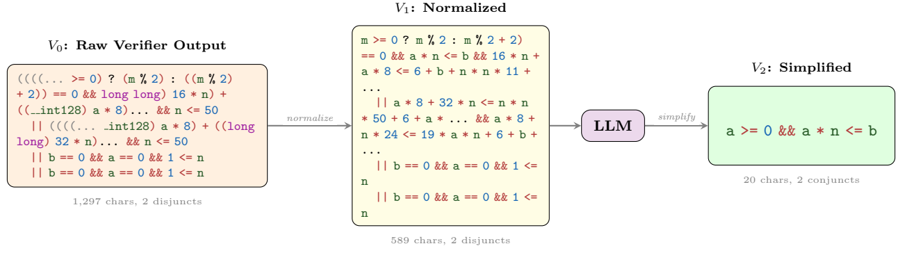
Figure 1: WONDA pipeline on 7241_2.c. The raw verifier output ( V_0 ) is normalized ( V_1 ); the LLM then merges parity-based case splits into a single linear inequality ( V_2 ): a \geq 0 \ \&\& \ a * n \leq b , a 65\times character reduction with 4.3\times verification speedup.
