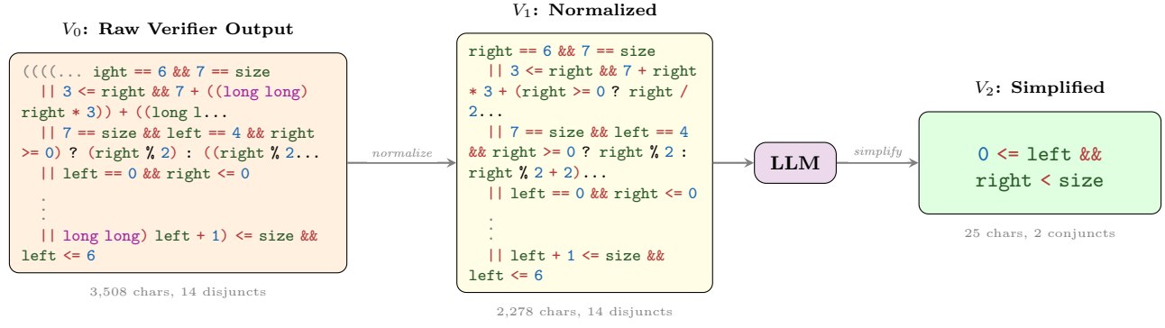
Figure 1: WONDA pipeline on 7861_1.c. The raw verifier output ( V_0 ) is normalized ( V_1 ); the LLM then removes size-specific overfitting and keeps valid binary-search index bounds ( V_2 ): 0 <= left && right < size , a 140× character reduction with 5.3 × verification speedup.
