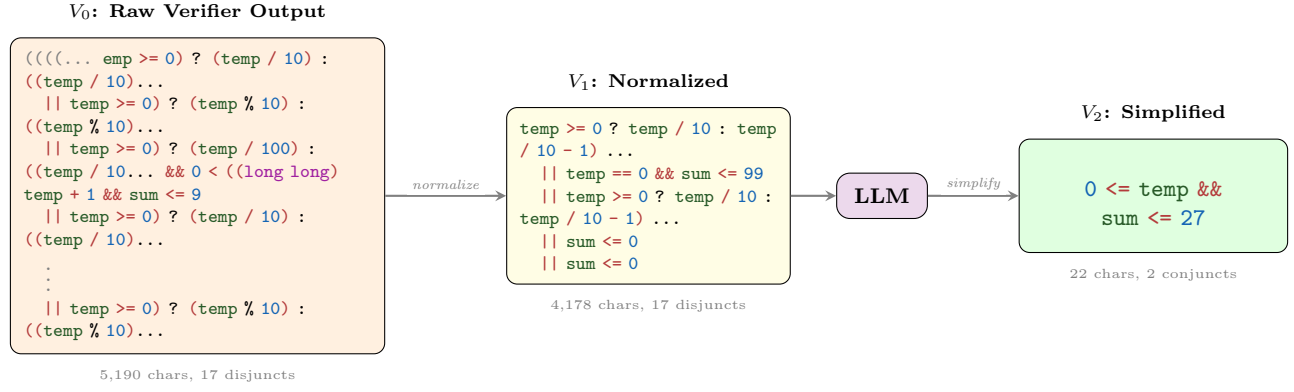
Figure 1: WONDA pipeline on 8353_1.c. The raw verifier output ( V_0 ) is normalized ( V_1 ); the LLM then bounds the digit-sum loop using the input magnitude and non-negativity ( V_2 ): 0 \leq \text{temp} \ \&\& \ \text{sum} \leq 27 , a 236\times character reduction with 1.2\times verification speedup.
