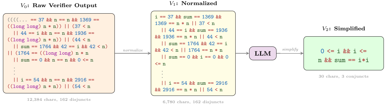
Figure 1: WONDA pipeline on 8694_1.c. The raw verifier output ( V_0 ) is normalized ( V_1 ); the LLM then recognizes the sum-of-odd-integers pattern and states the i^2 closed form ( V_2 ): 0 \leq i \ \&\& \ i \leq n \ \&\& \ \text{sum} == i*i , a 413× character reduction with 22.5 × verification speedup.
