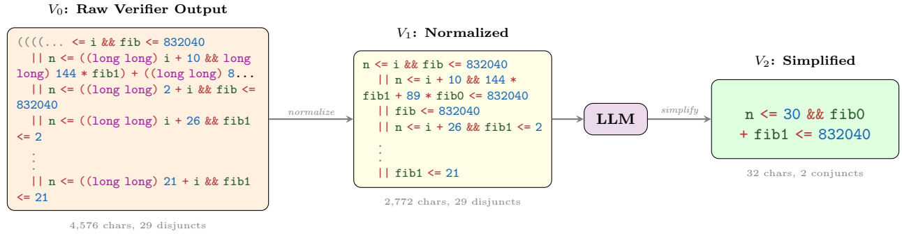
Figure 1: WONDA pipeline on 905_1.c. The raw verifier output ( V_0 ) is normalized ( V_1 ); the LLM then drops redundant Fibonacci case bounds while keeping the needed growth limit ( V_2 ): n \leq 30 \ \&\& \ fib0 + fib1 \leq 832040 , a 143 \times character reduction with verified correct & sufficient.
