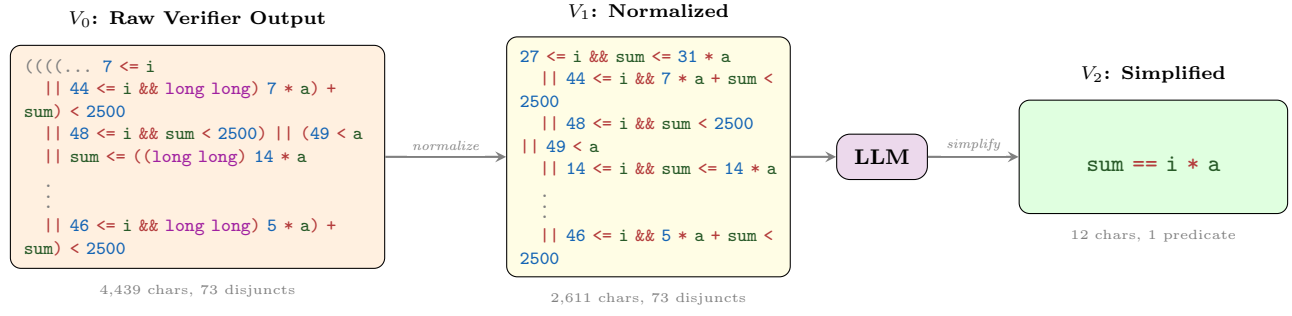
Figure 1: WONDA pipeline on 9136_1.c. The raw verifier output ( V_0 ) is normalized ( V_1 ); the LLM then replaces case enumeration with the linear relation between sum and the loop counter ( V_2 ): sum == i * a , a 370 \times character reduction with 3.8 \times verification speedup.
