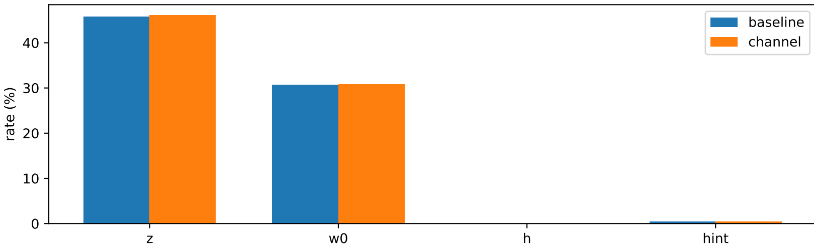
ML-DSA-65 reject rates per attempt
