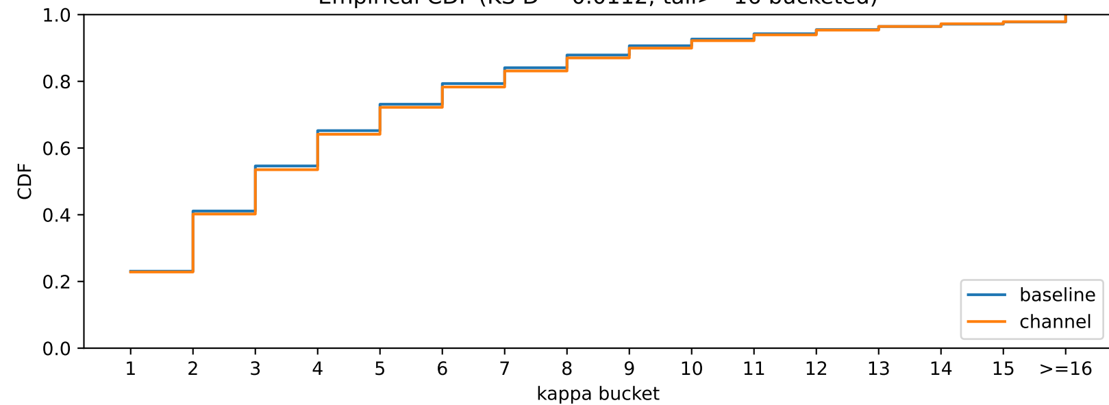
Empirical CDF (KS D = 0.0112; tail \geq 16 bucketed)
