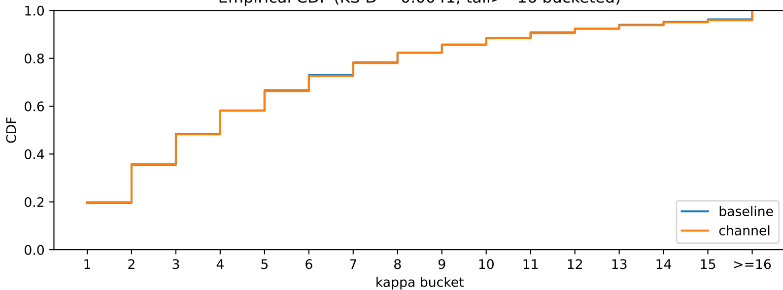
Empirical CDF (KS D = 0.0041; tail \geq 16 bucketed)
