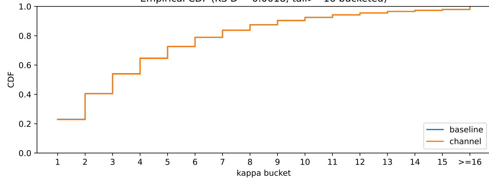
Empirical CDF (KS D = 0.0018; tail \geq 16 bucketed)
