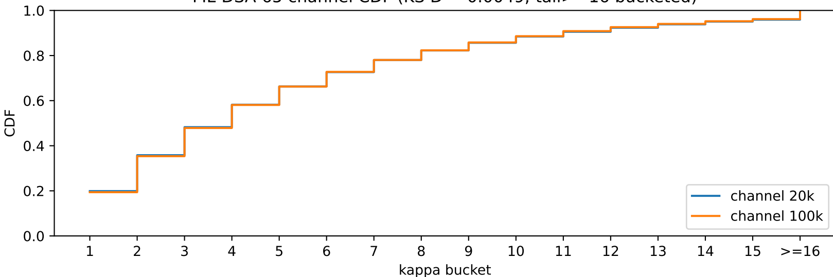
ML-DSA-65 channel CDF (KS D = 0.0049; tail \geq 16 bucketed)
