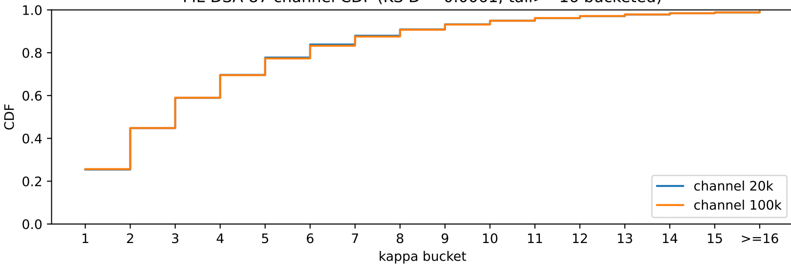
ML-DSA-87 channel CDF (KS D = 0.0061; tail \geq 16 bucketed)
