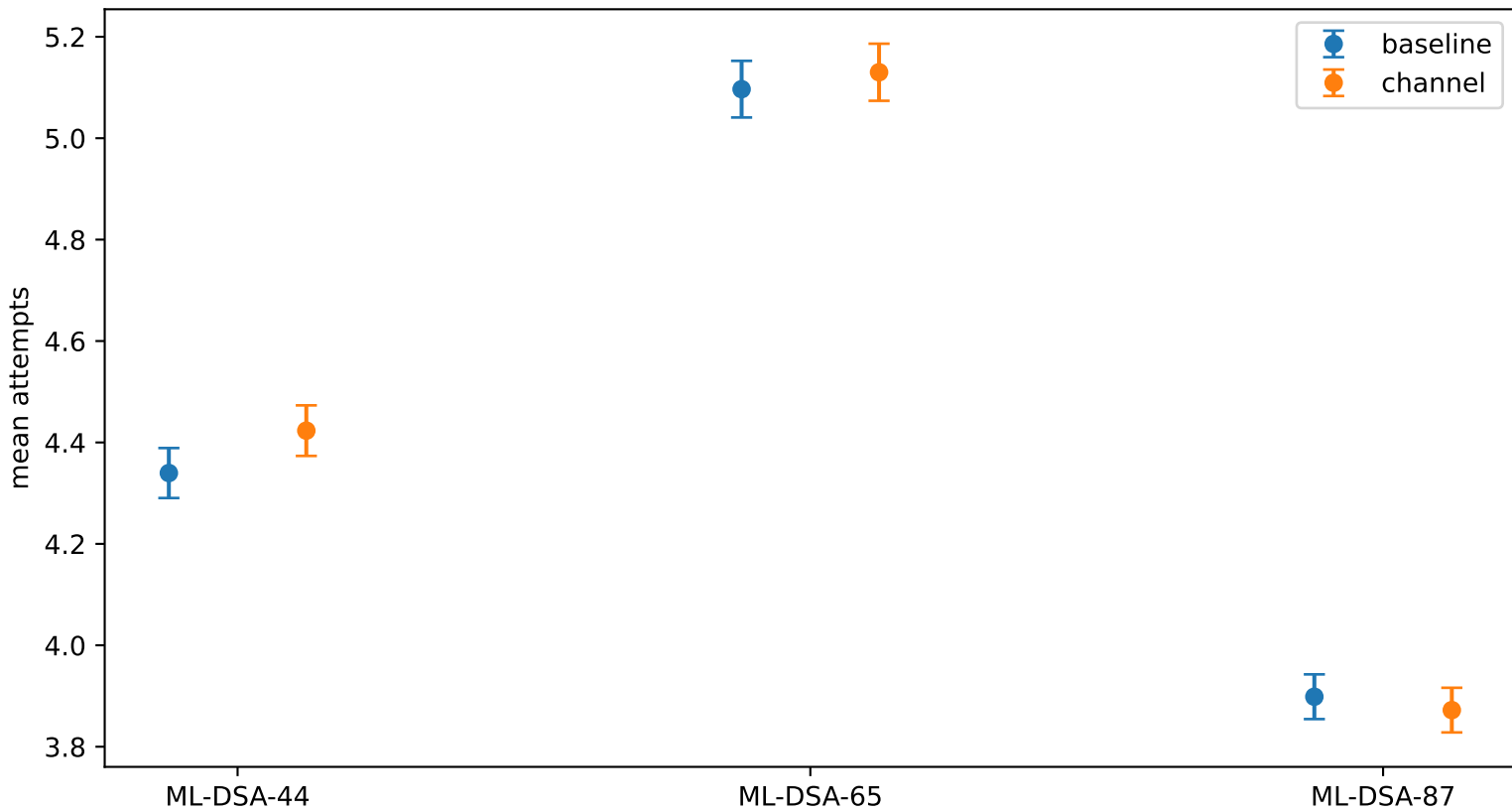
Mean attempts with 95% CI (tail \geq 16- \rightarrow 16)
