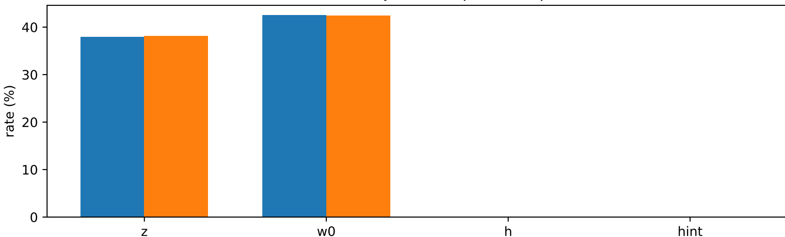
ML-DSA-87 reject rates per attempt
