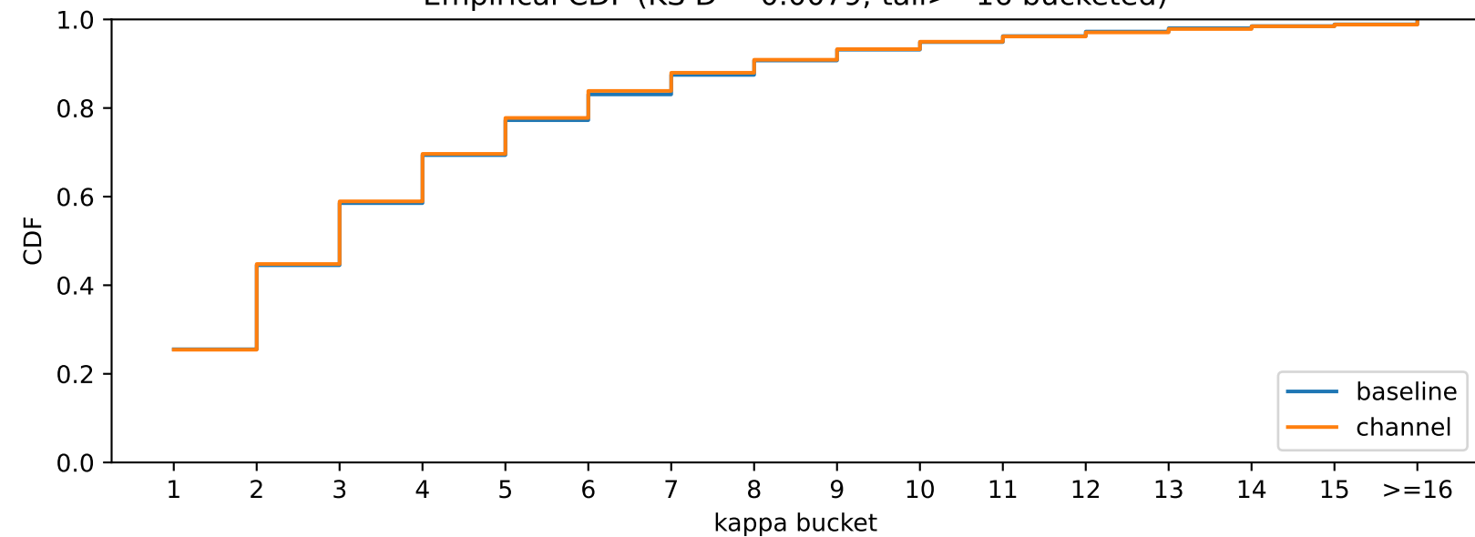
Empirical CDF (KS D = 0.0079; tail \geq 16 bucketed)
