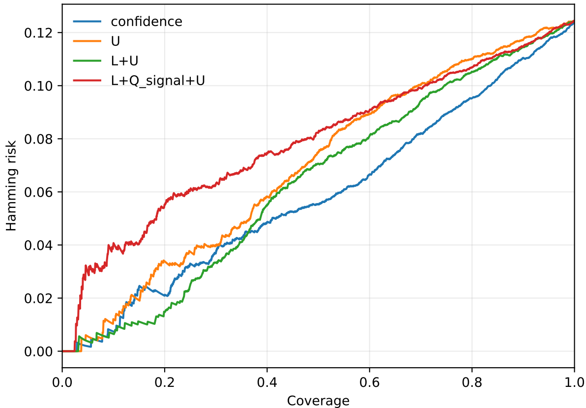
Risk-coverage: baseline wander severe
