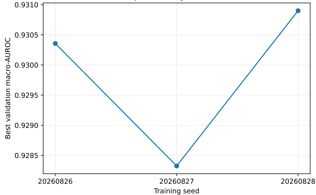
Baseline reproducibility across three seeds
