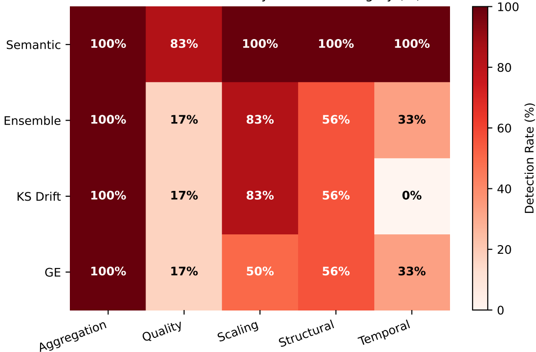
Detection Performance by Mutation Category (%)
