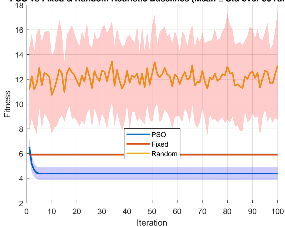
PSO vs Fixed & Random Heuristic Baselines (Mean \pm Std over 30 runs)
