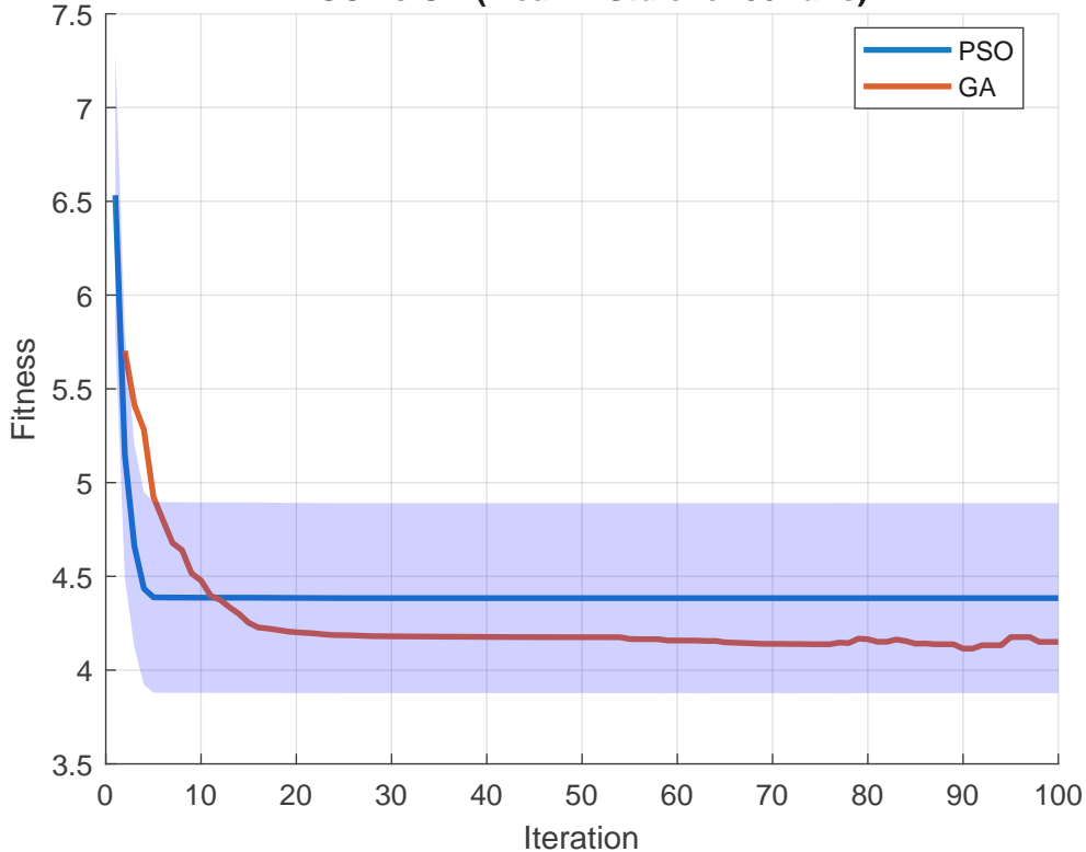
PSO vs GA (Mean \pm Std over 30 runs)
