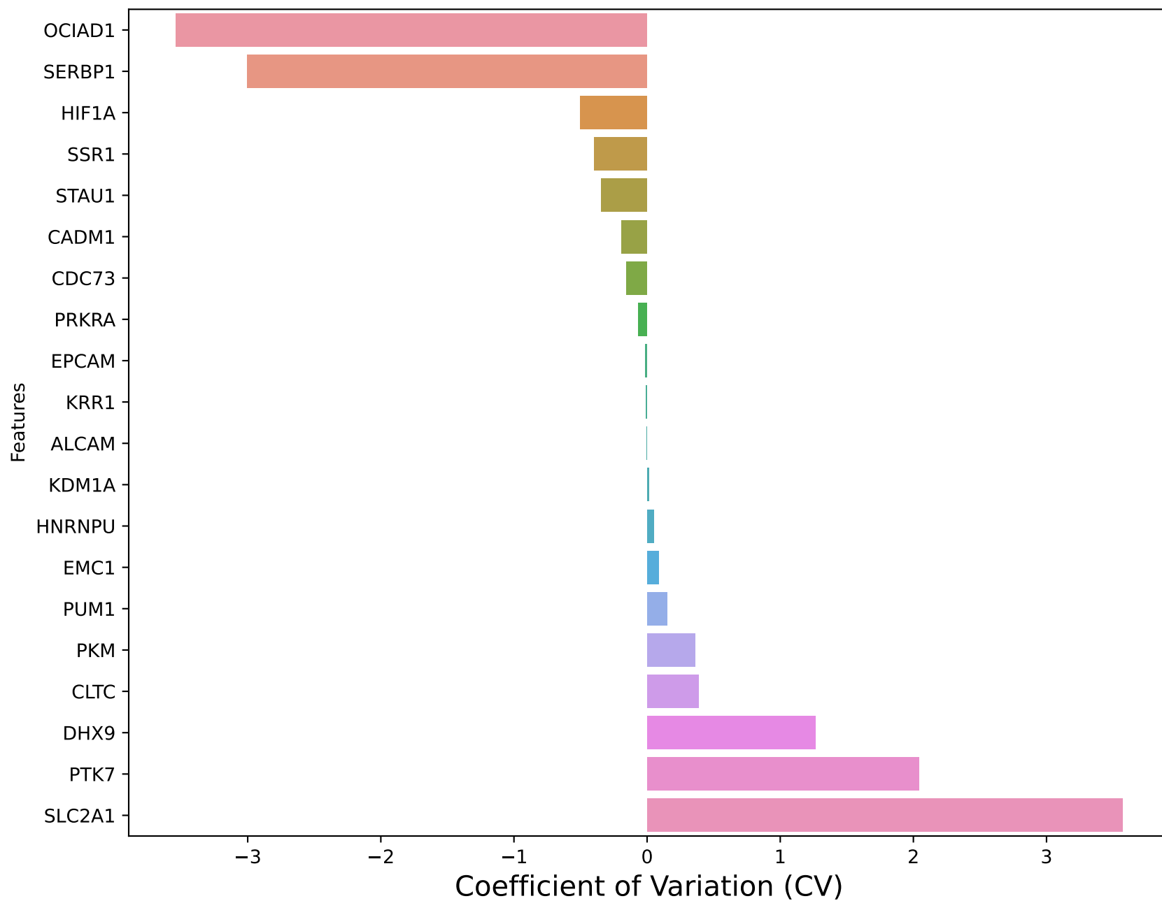
Coefficient of Variation of SHAP Values Across Folds for LUAD
