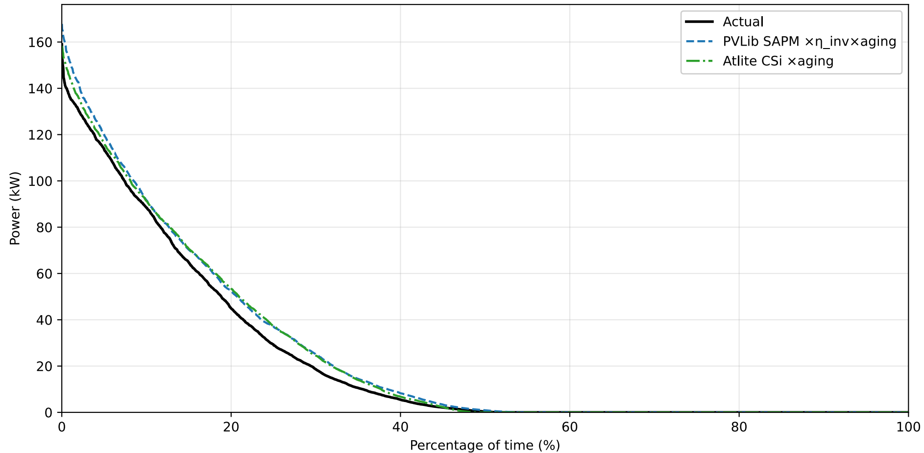
Jülich PV 2023 — hourly generation duration curve (n=8760 hours; sims include inverter/aging derates)
