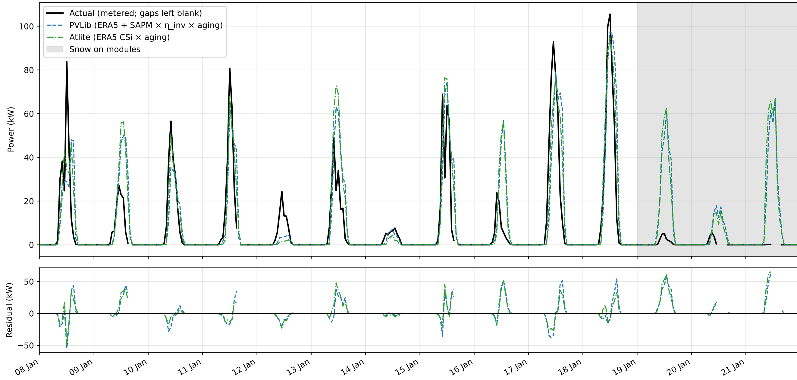
Campus Jülich PV, 8-21 January 2023 (matched ERA5; inverter/aging derates)
