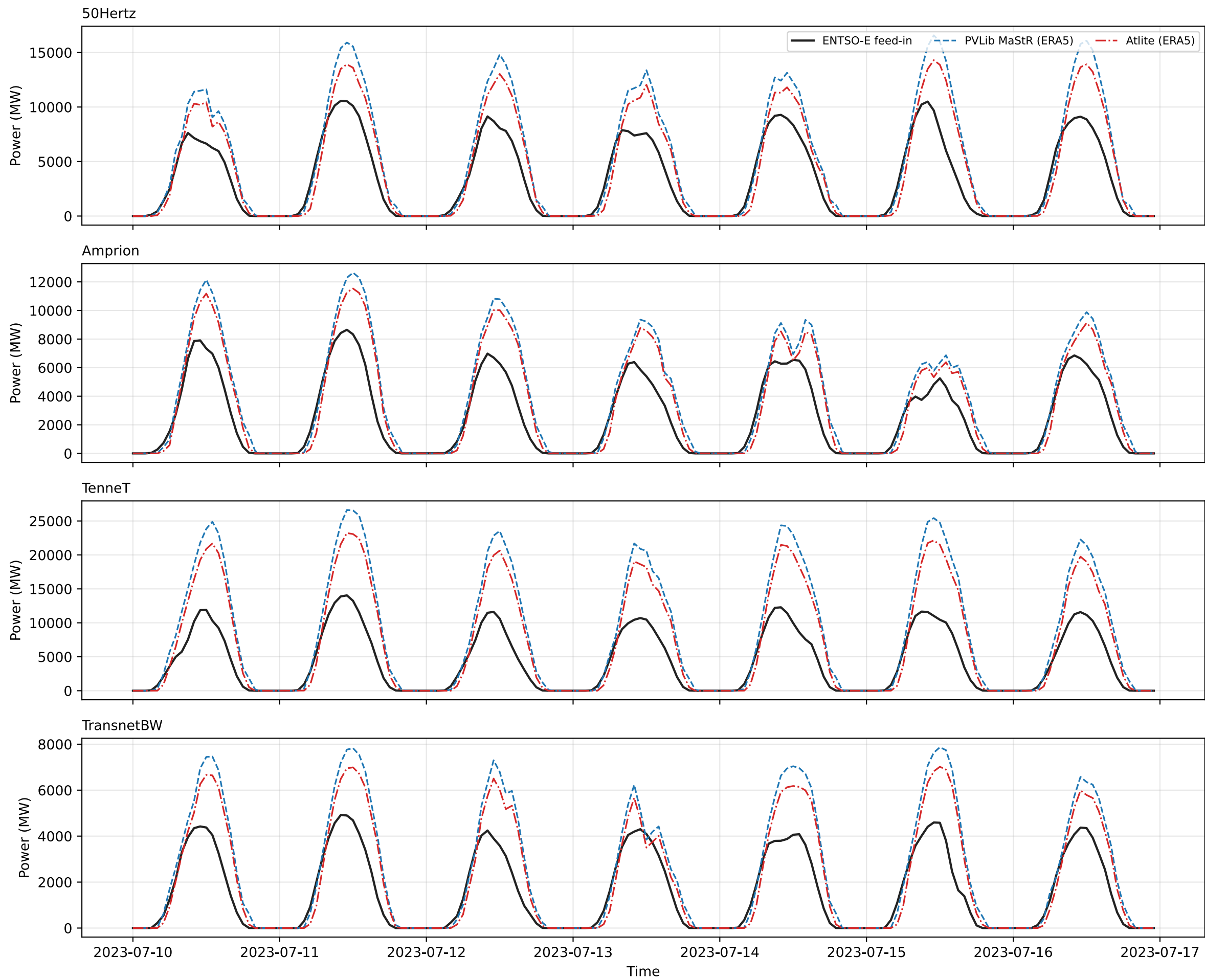
German TSO solar — matched ERA5 sample week 2023-07-10 to 2023-07-16
