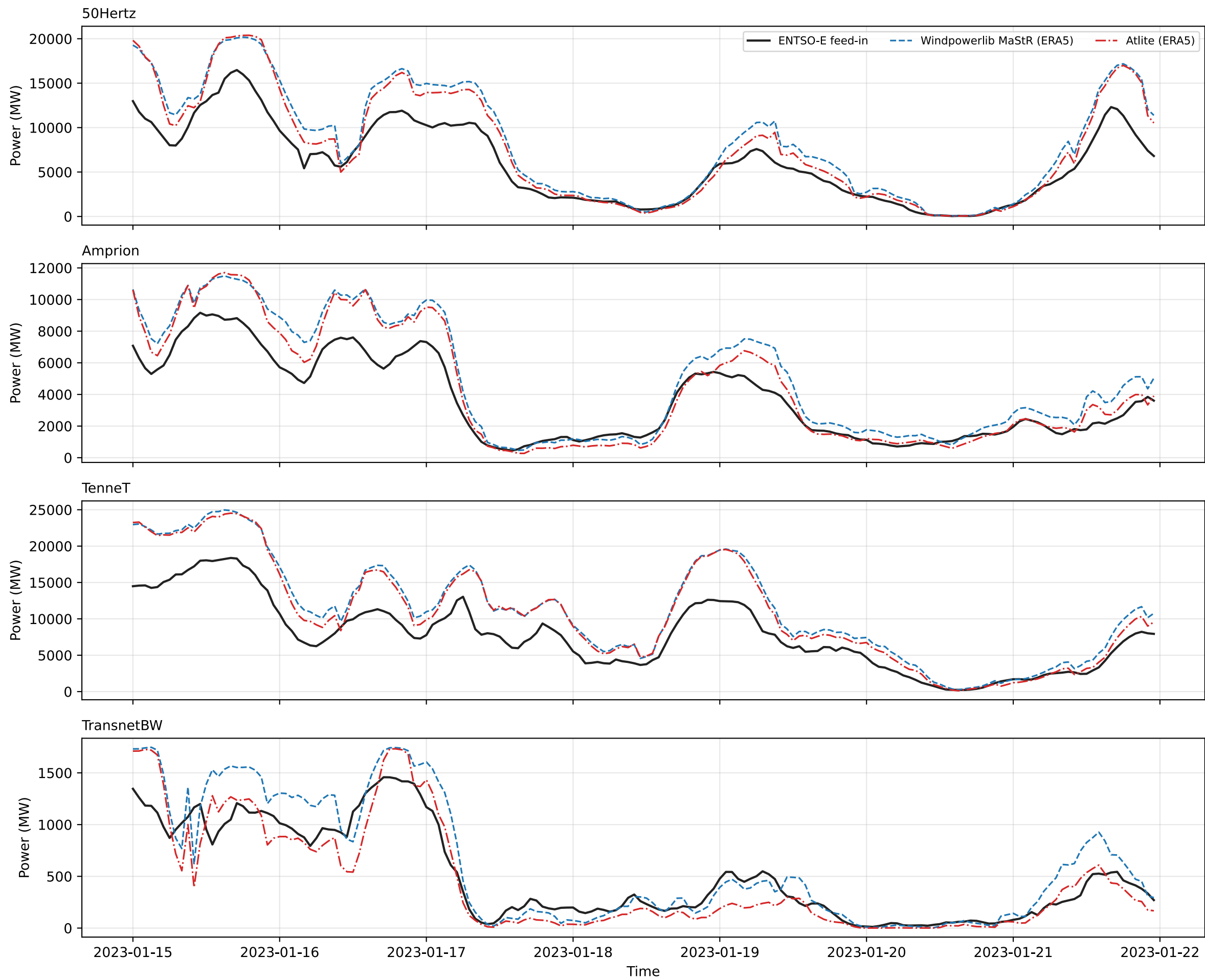
German TSO onshore wind — matched ERA5 sample week 2023-01-15 to 2023-01-21
