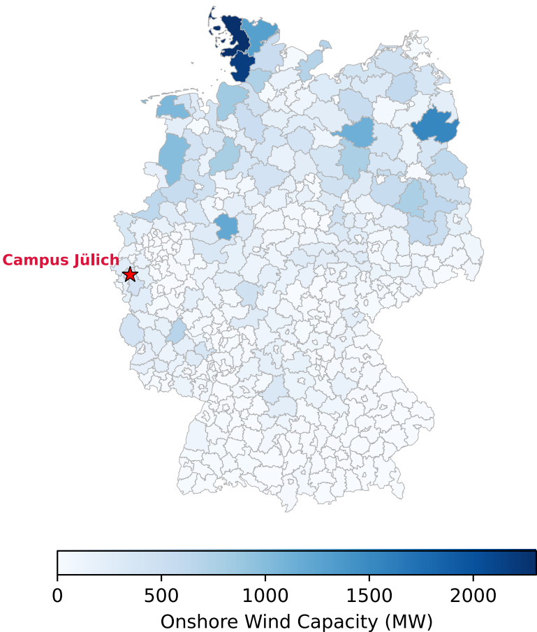
German Onshore Wind Fleet (MaStR 2023)
